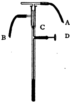
FIG. 115.—Reichert's thermo-regulator.
